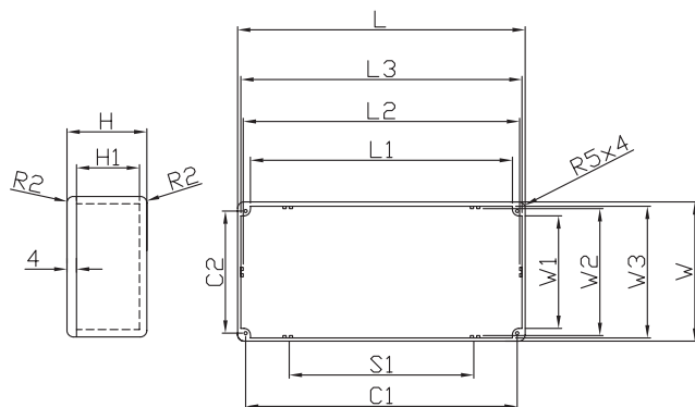
Dimension Table
