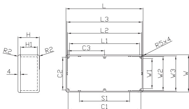
Dimension Table
