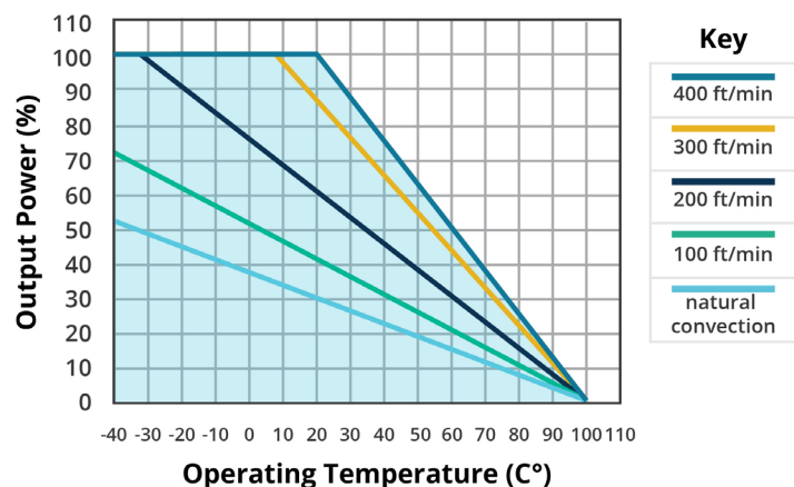
TEMPERATURE DERATING CURVE PRC300-300-S5
