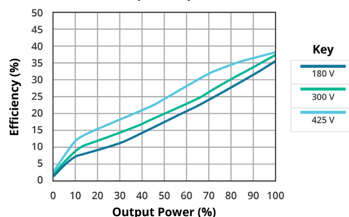
POWER DISSIPATION VS OUTPUT POWER PRC300-300-S12 (at 25°C)
