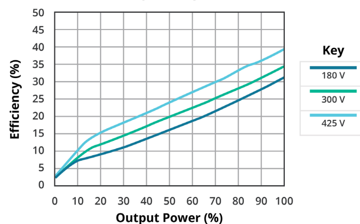
POWER DISSIPATION VS OUTPUT POWER PRC300-300-S24 (at 25°C)
