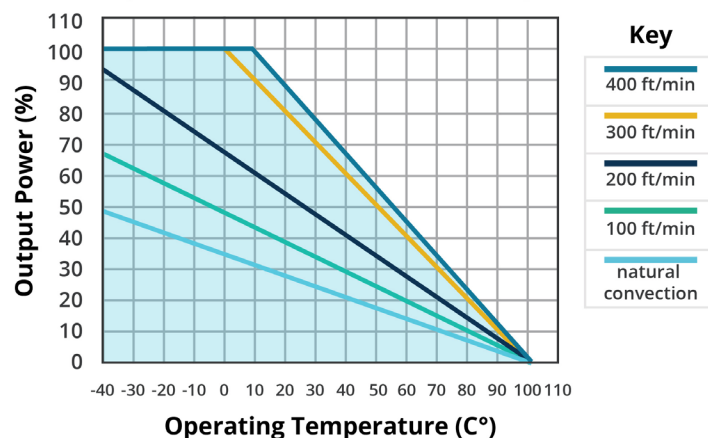
TEMPERATURE DERATING CURVE PRC300-300-S12
